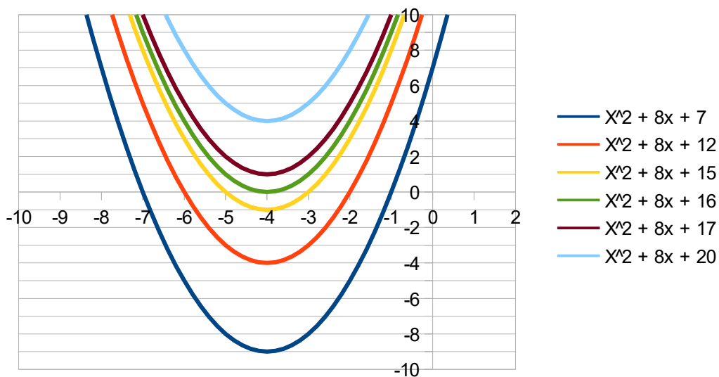
Figure 8: Graphs of the six various parabolas
