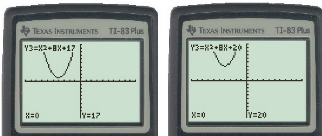
Figure 7: Graph of parabolas from multiplied imaginary lines.
