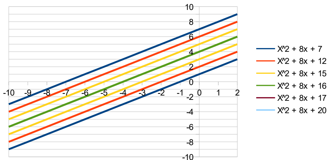
Figure 9: Graphs of the pairs of lines multiplied to form various parabolas
