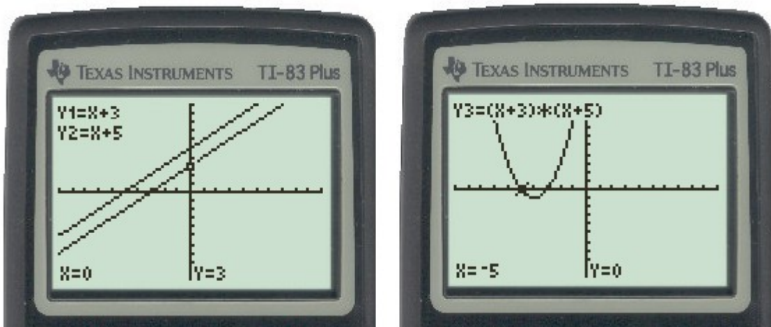
Figure 5: Graph of x + 3 and x + 5 and their resulting parabola
