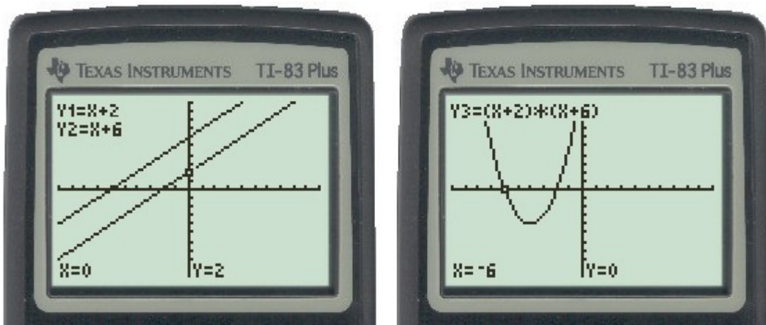
Figure 4: Graph of x + 2 and x + 6 and their resulting parabola
