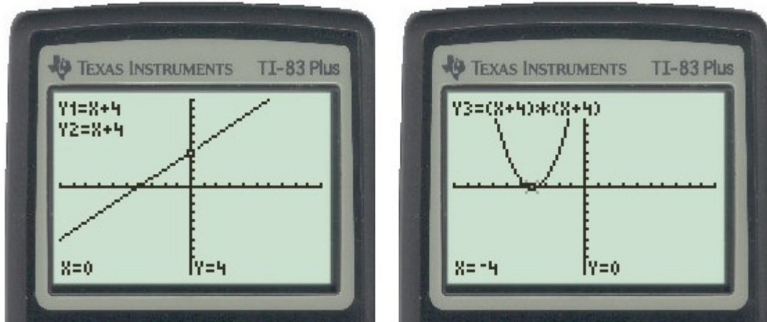
Figure 6: Graph of x + 4 squared and the resulting parabola
