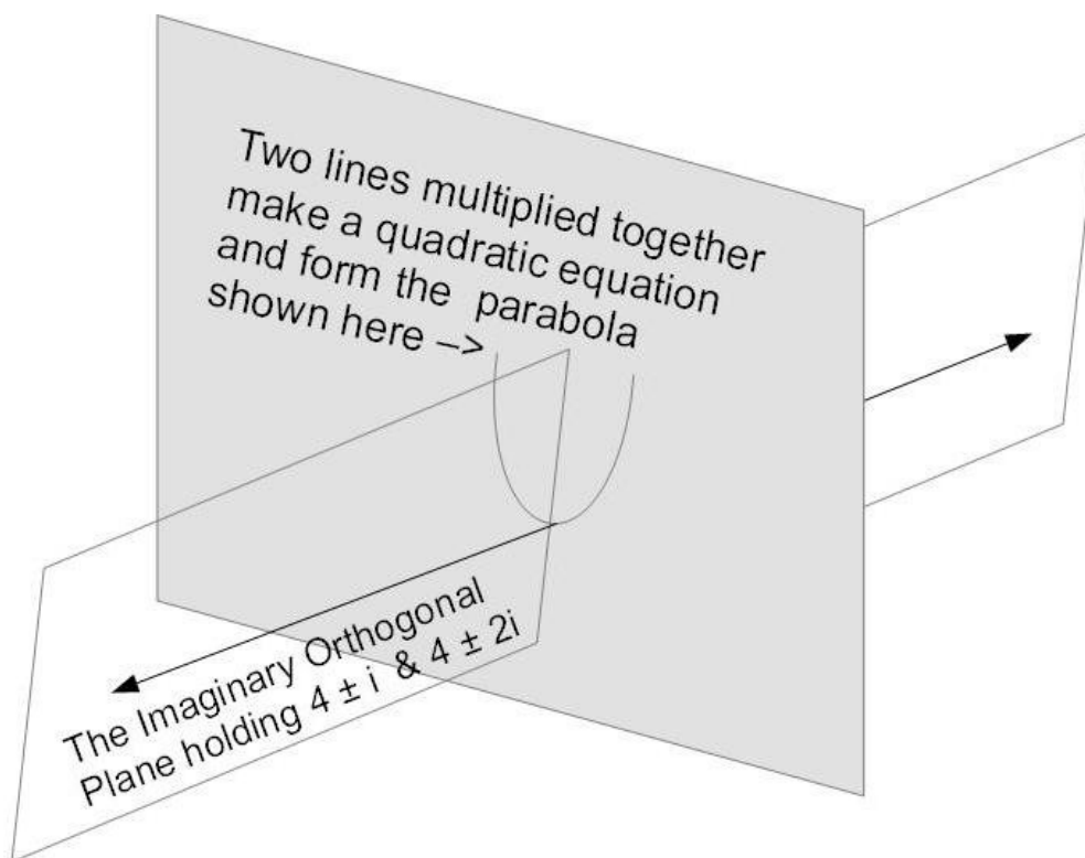
Figure 10: Graphic of a plane orthogonal to the blackboard.
