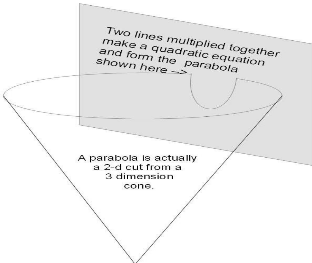
Figure 1: A cone forms a parabola
