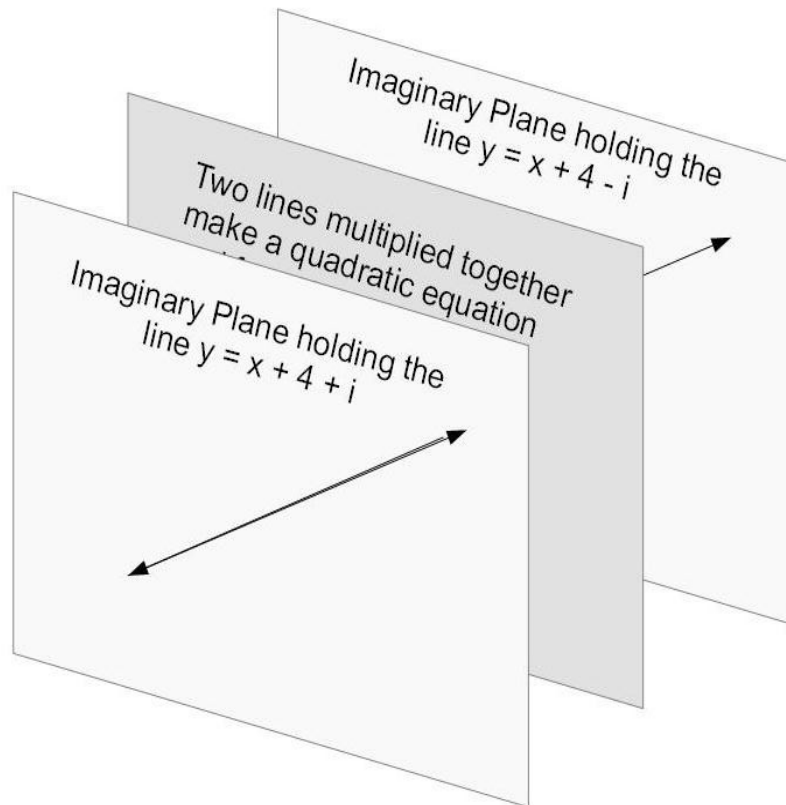
Figure 11: Graphic of the imaginary planes relative to the blackboard
