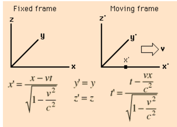
Figure 15 Fixed Frame to Moving Frame of the Lorentz Transformation
