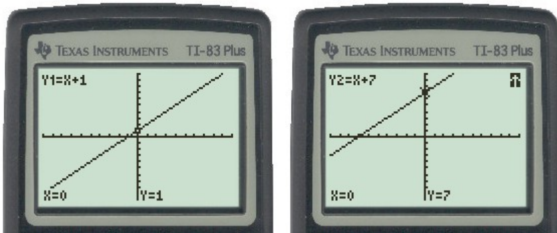
Figure 2: Graph of lines x + 1 and x + 7
