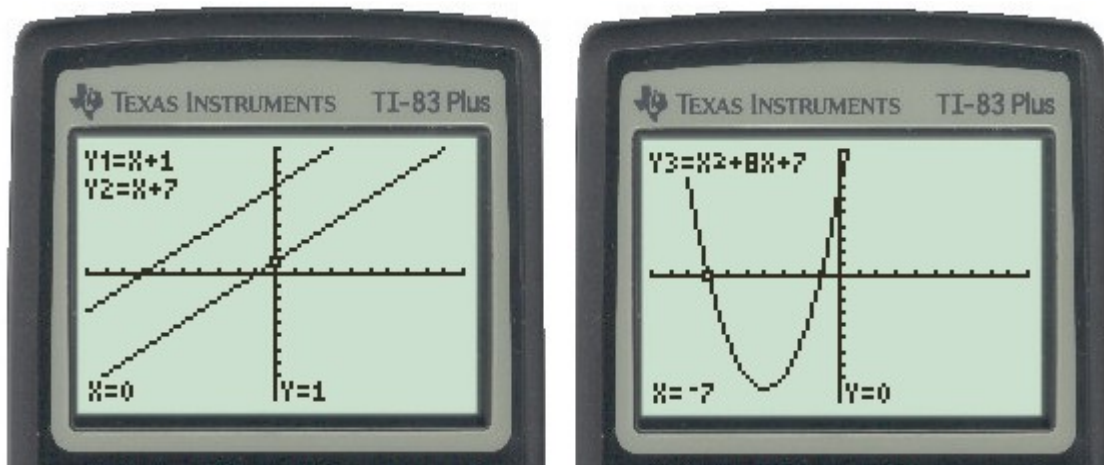
Figure 3: Graph of x + 1 and x + 7 and their resulting parabola
